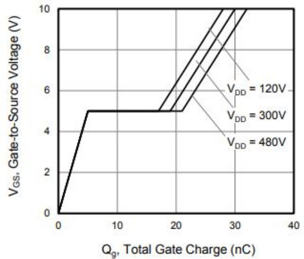
Figure 8. Gate Charge
