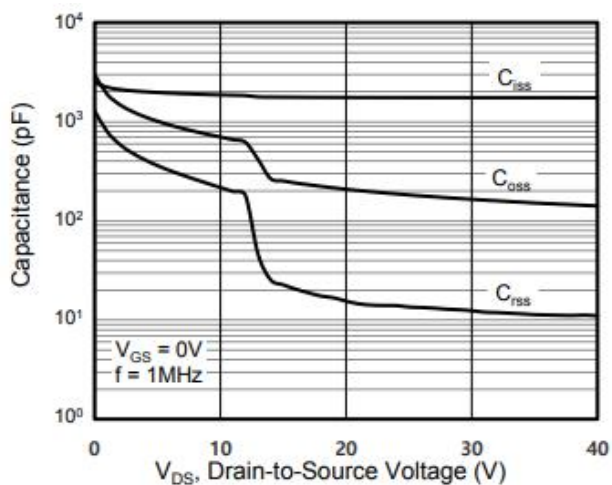
Figure 7. Capacitance
