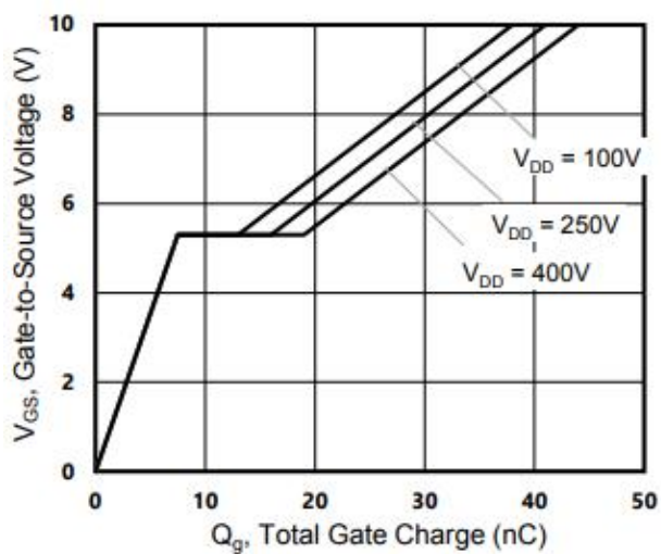
Figure 8. Gate Charge
