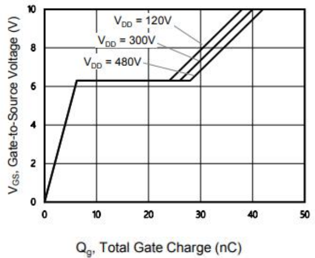
Figure 8. Gate Charge
