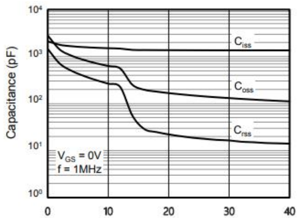
Figure 7. Capacitance
