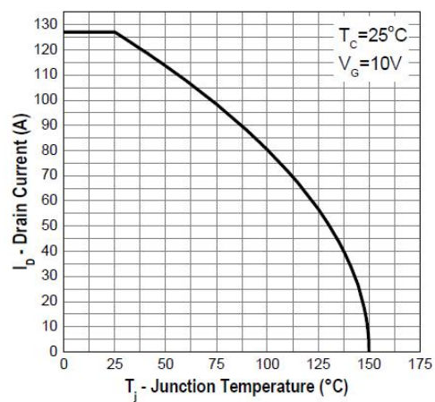
Drain Current
