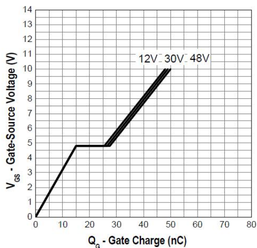
Gate Charge
