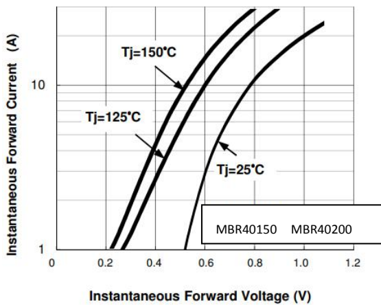
Figure 8. Typical Forward Characteristics
