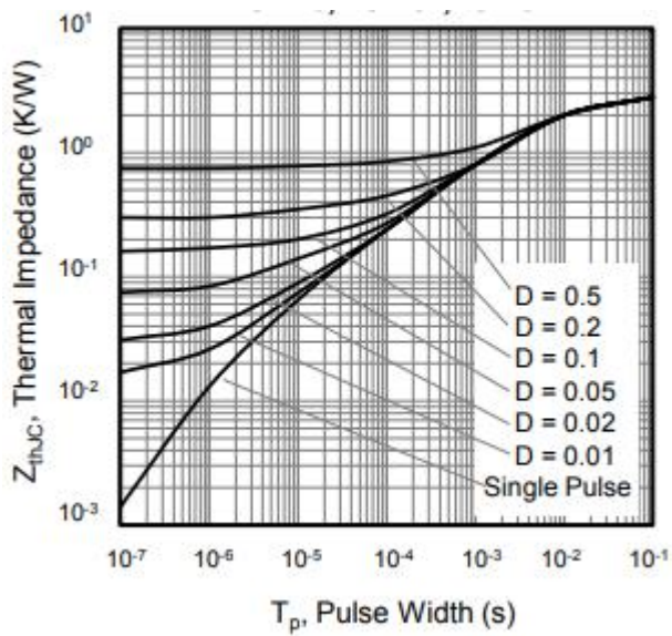
Figure 9. Transient Thermal Impedance TO-251, TO-252
