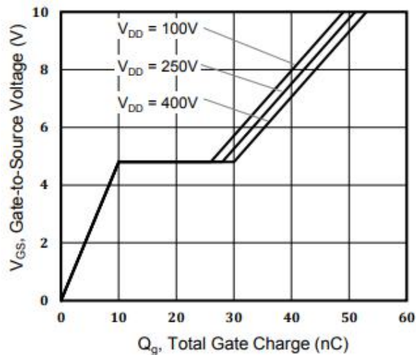
Figure 8. Gate Charge
