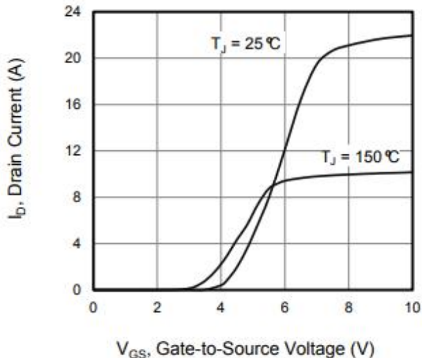
Figure 5. Transfer Characteristics
