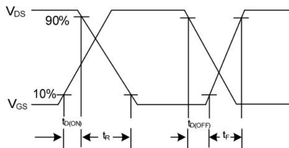
Switching Waveforms
