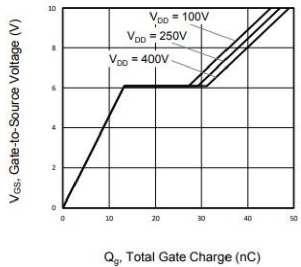
Figure 8. Gate Charge
