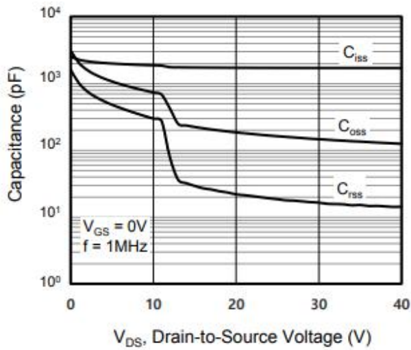
Figure 7. Capacitance
