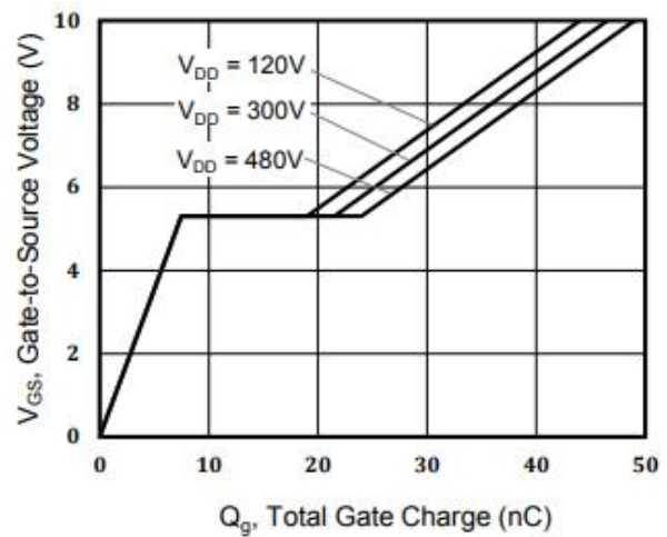
Figure 8. Gate Charge
