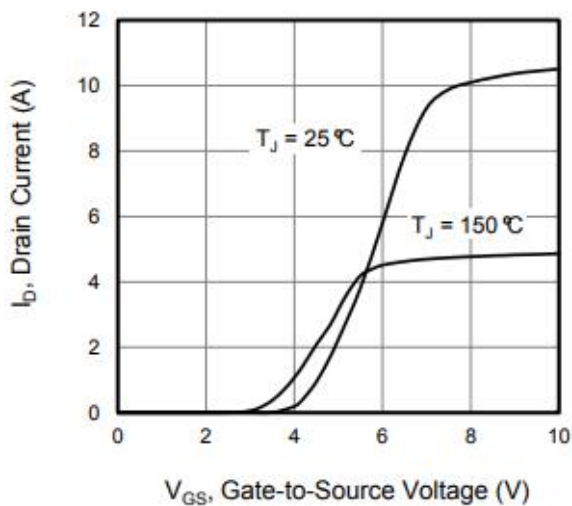
Figure 5. Transfer Characteristics
