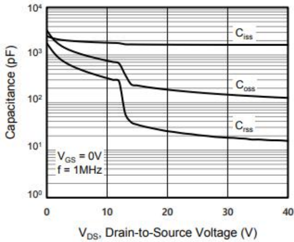
Figure 7. Capacitance
